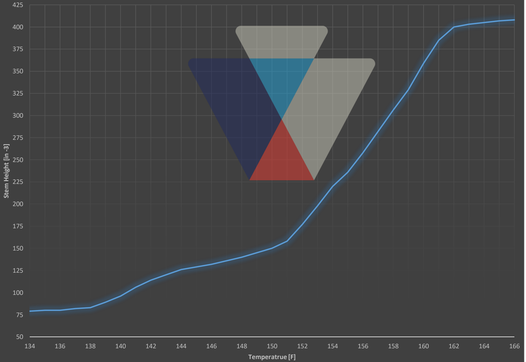
Temperature vs. Stem Height - P77SH 162F
