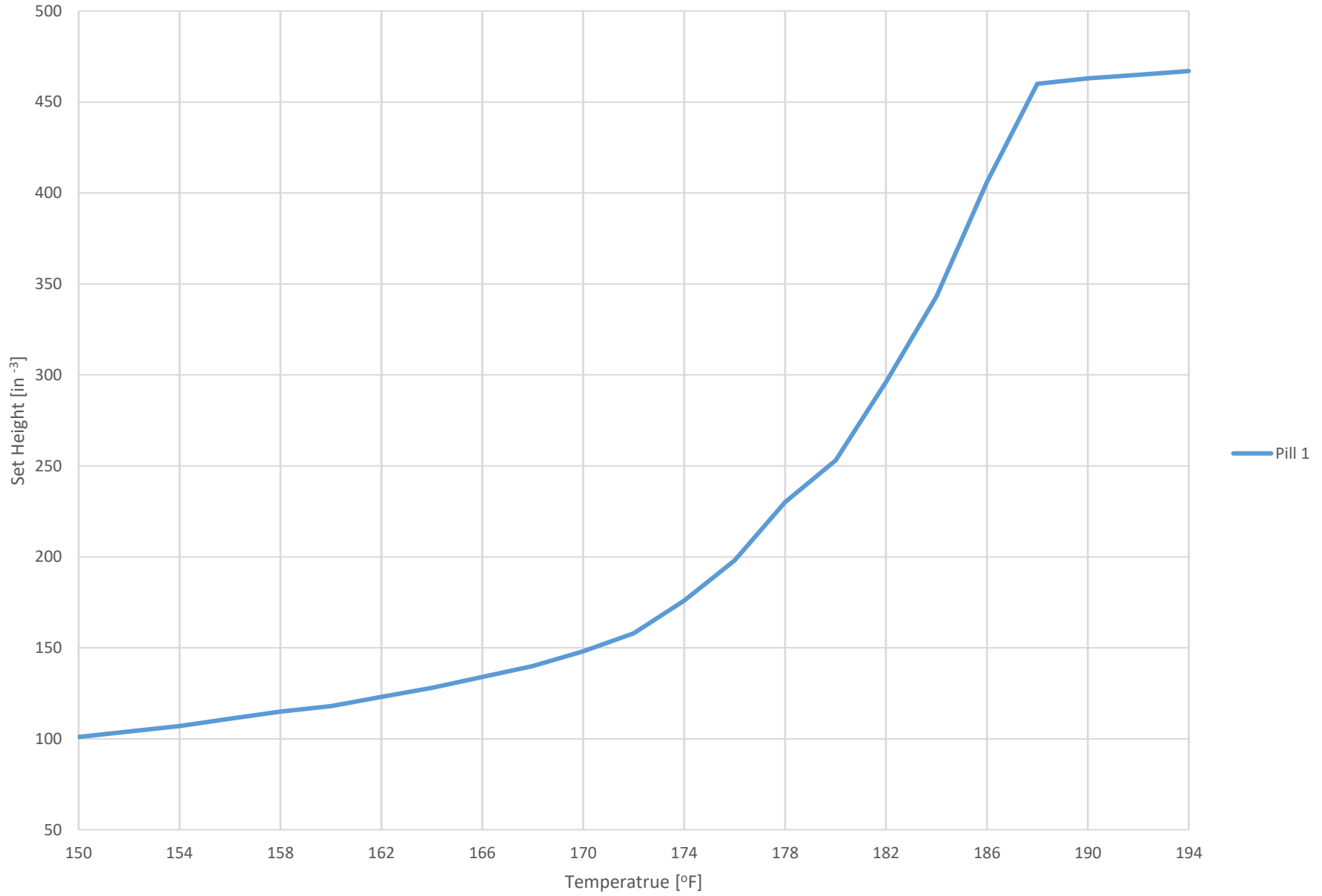
Temperature vs. Stem Height - MS 9134 190F
