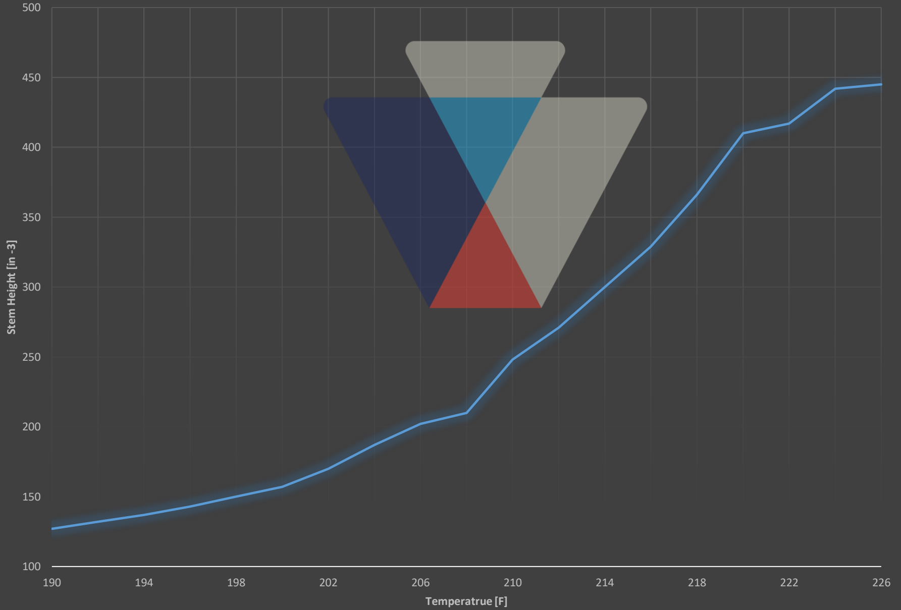
Temperature vs. Stem Height - MS 9404 225F
